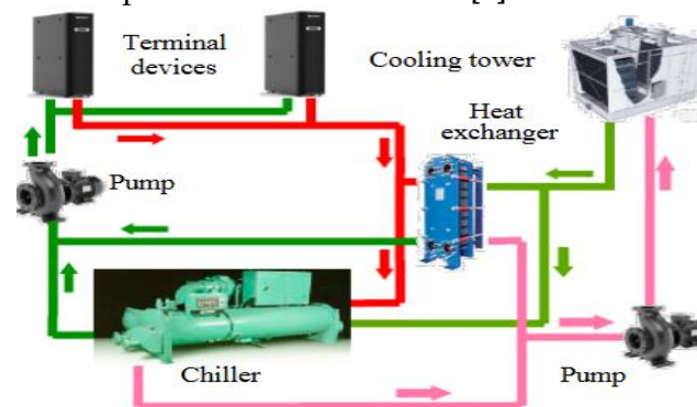
Fig. 5. Water-based free cooling system
