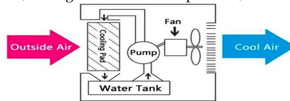
Fig. 4. Evaporative cooling system
